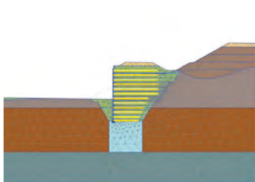
Prediction of structural deformation (FEM Analysis)
